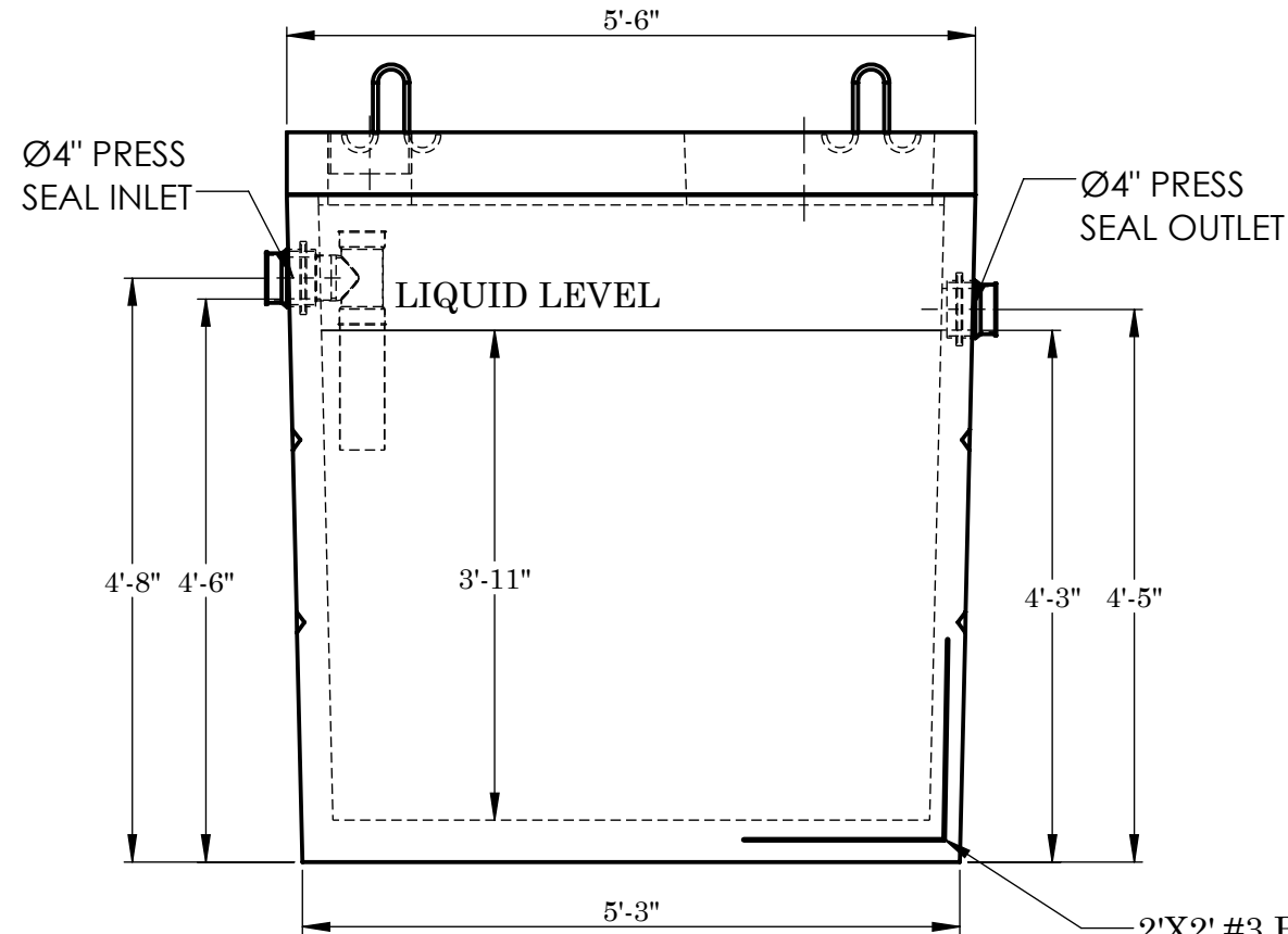
FRONT VIEW
