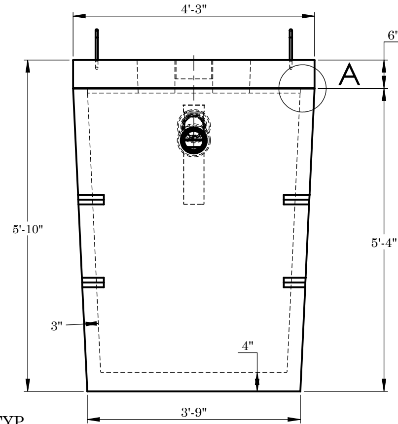
SIDE VIEW
