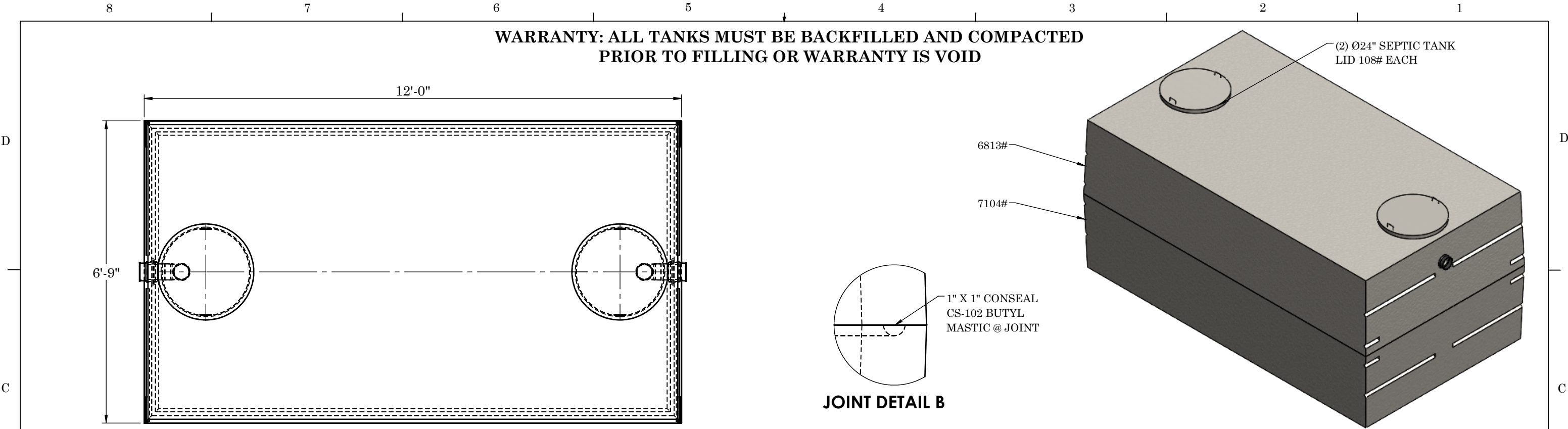
TOP VIEW
