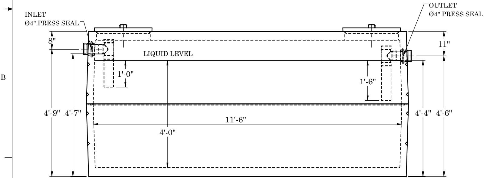
FRONT VIEW
