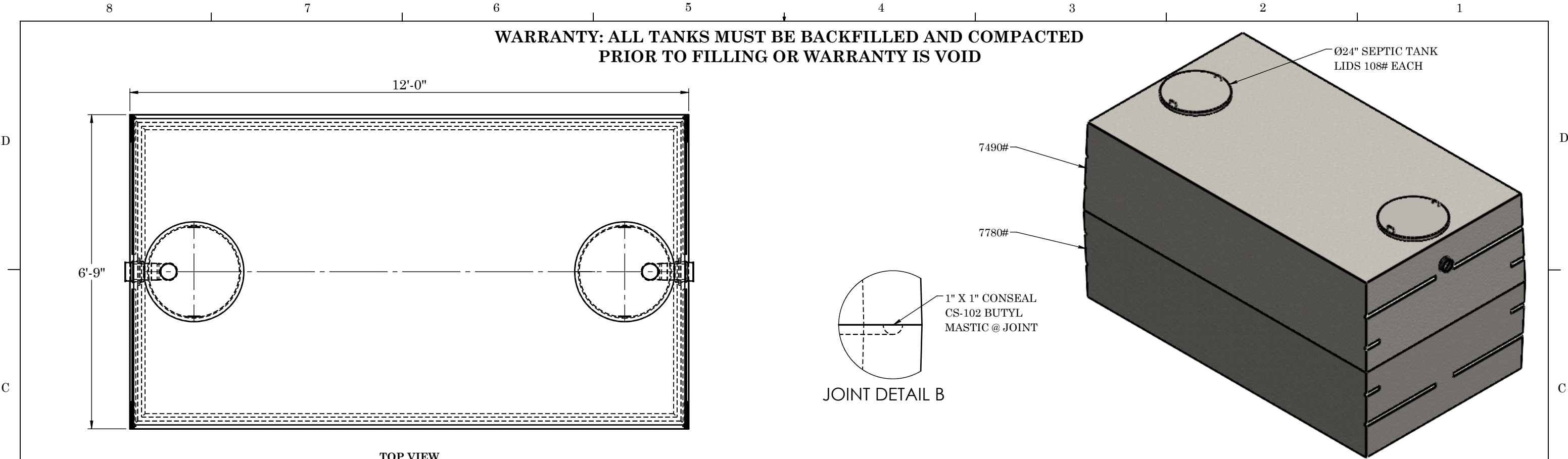
TOP VIEW
