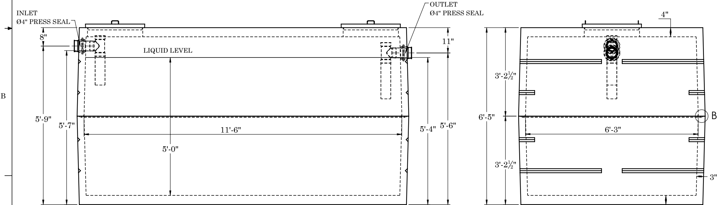
FRONT VIEW
