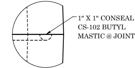
JOINT DETAIL B
