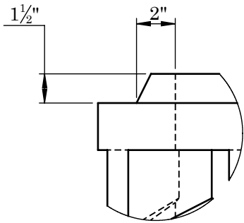
SHIPLAP DETAIL B
