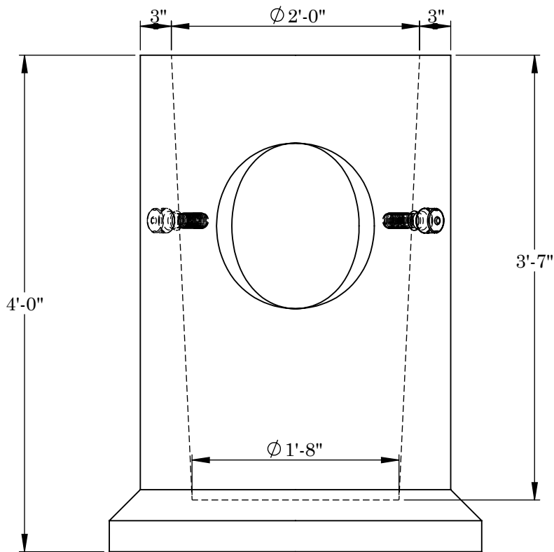
FRONT VIEW
