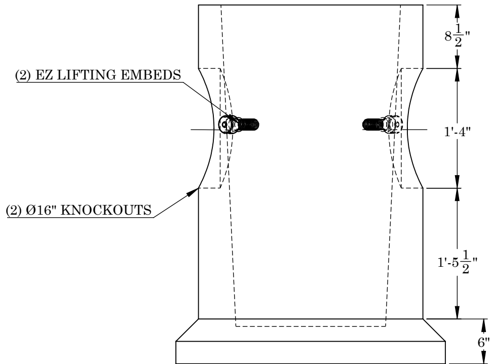
SIDE VIEW
