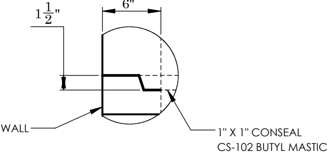
SHI LAP JOINT DETAIL B
