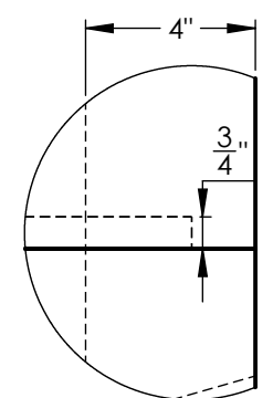
SHIPLAP DETAIL D
