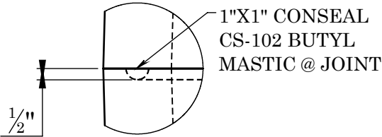
JOINT DETAIL B
