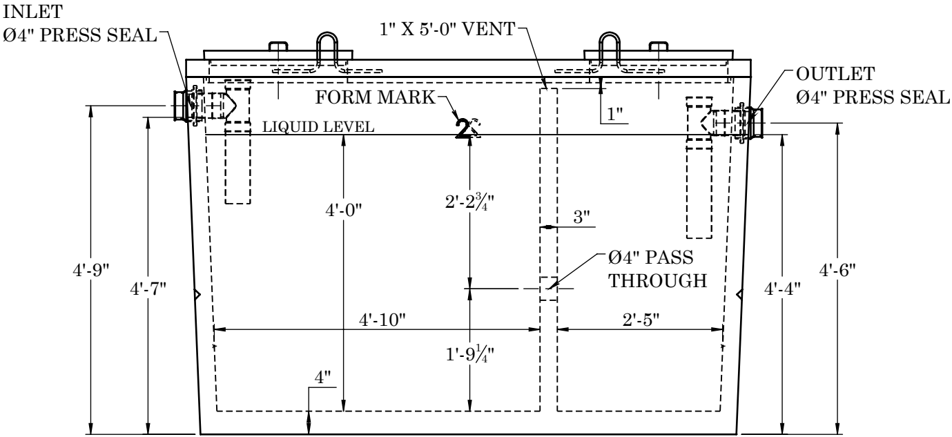
FRONT VIEW
