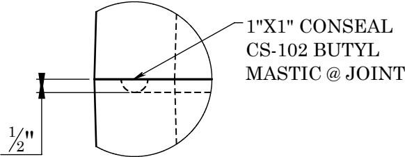
JOINT DETAIL B
