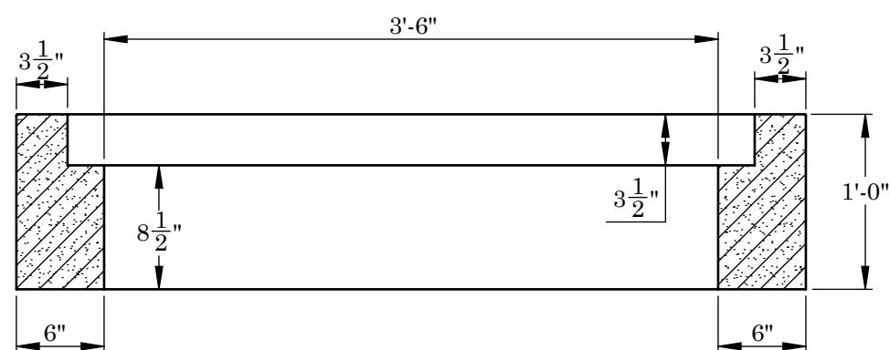
SIDE VIEW SECTION A-A
