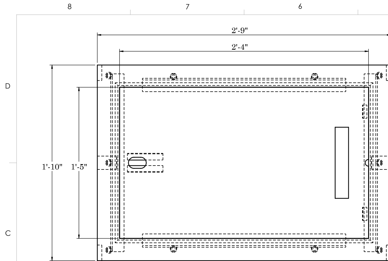
TOP VIEW
