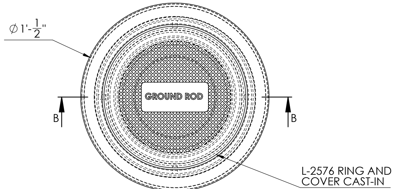
TOP VIEW
