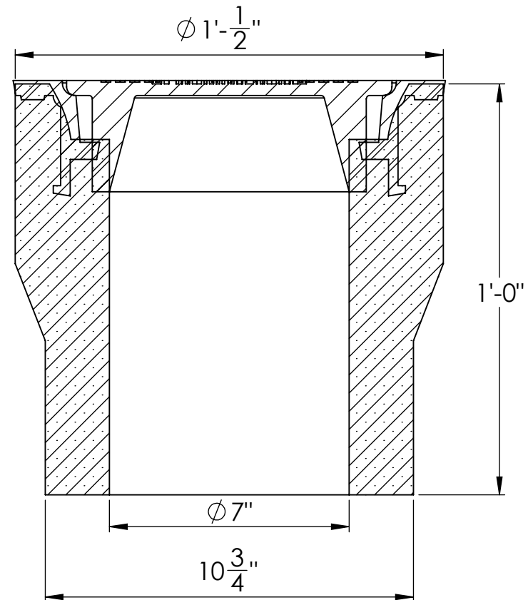
SECTION B-B
