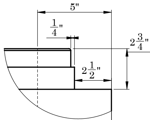
SHIPLAP DETAIL A
