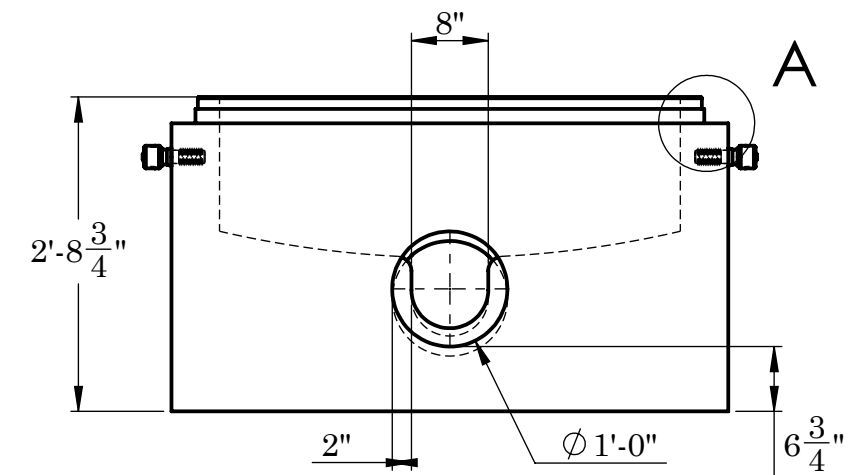
BACK VIEW
