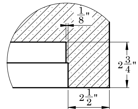
SHIPLAP DETAIL C
