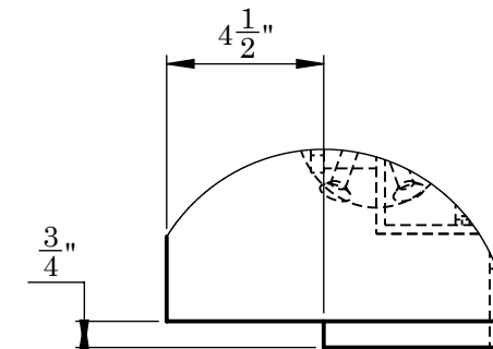
SHIPLAP DETAIL A
