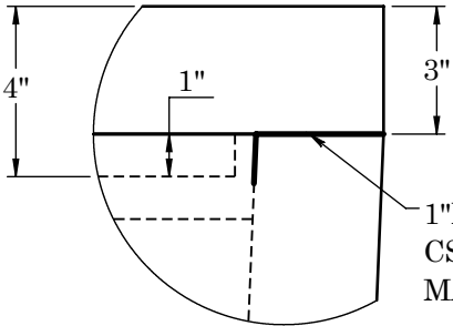
SHIPLAP DETAIL A
