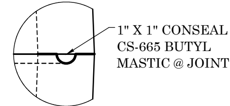
JOINT DETAIL B
