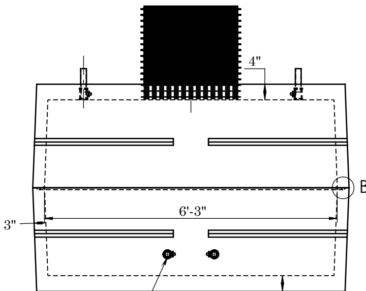
Ø1" GALV FITTINGS SIDE VIEW
