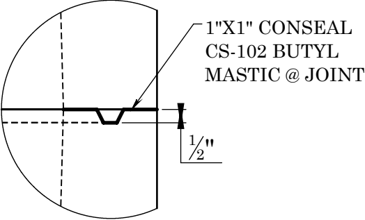
JOINT DETAIL B
