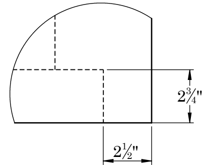
SHIPLAP DETAIL B
