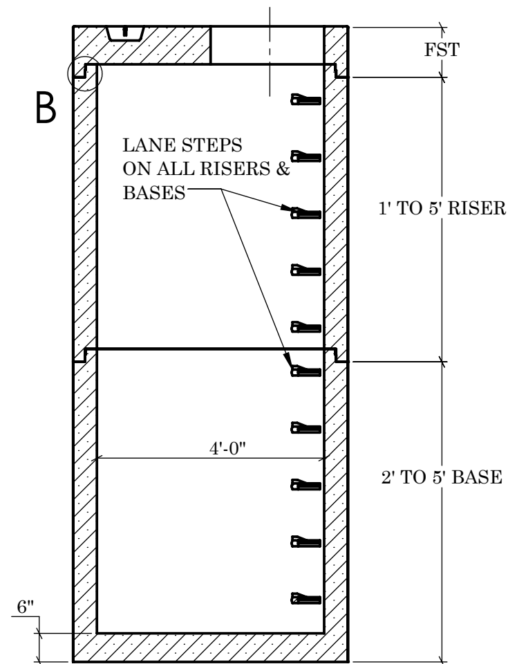
SIDE SECTION VIEW A-A
