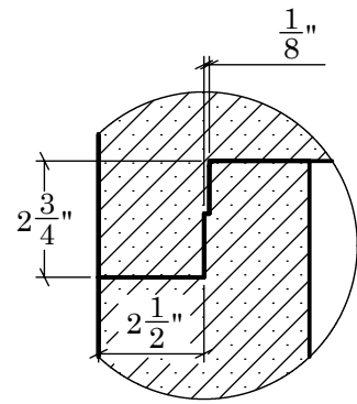
JOINT DETAIL B
