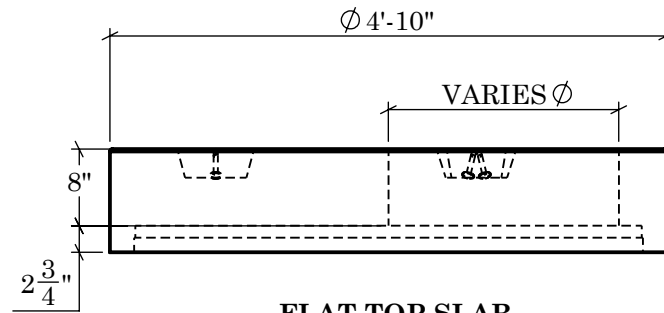
FLAT TOP SLAB PRODUCT #480F
