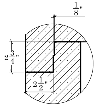
SHILAP DETAIL B
