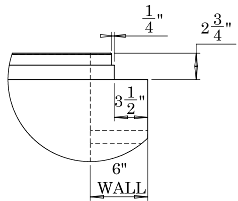
SHIPLAP DETAIL B (SAME FOR ALL SIZES)
