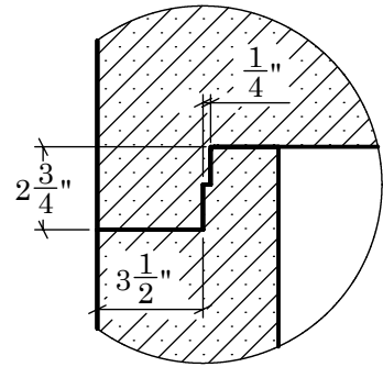
SHIPLAP DETAIL B
