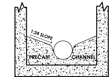
OPTIONAL PRECAST CHANNEL
