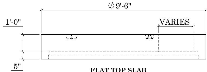
FLAT TOP SLAB PRODUCT #960F
