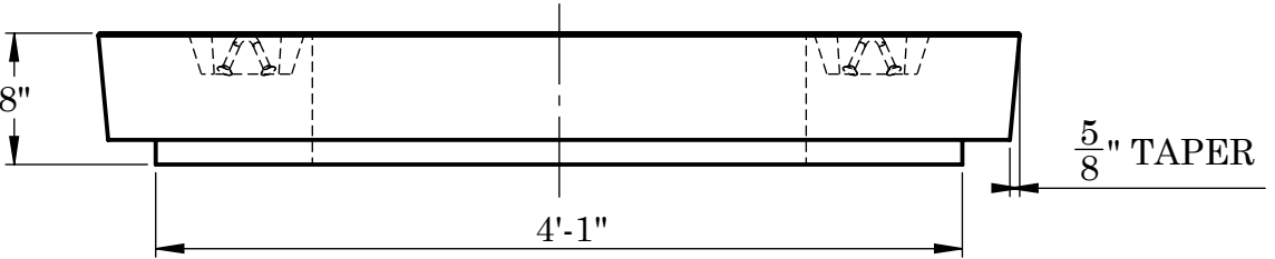
FRONT VIEW
