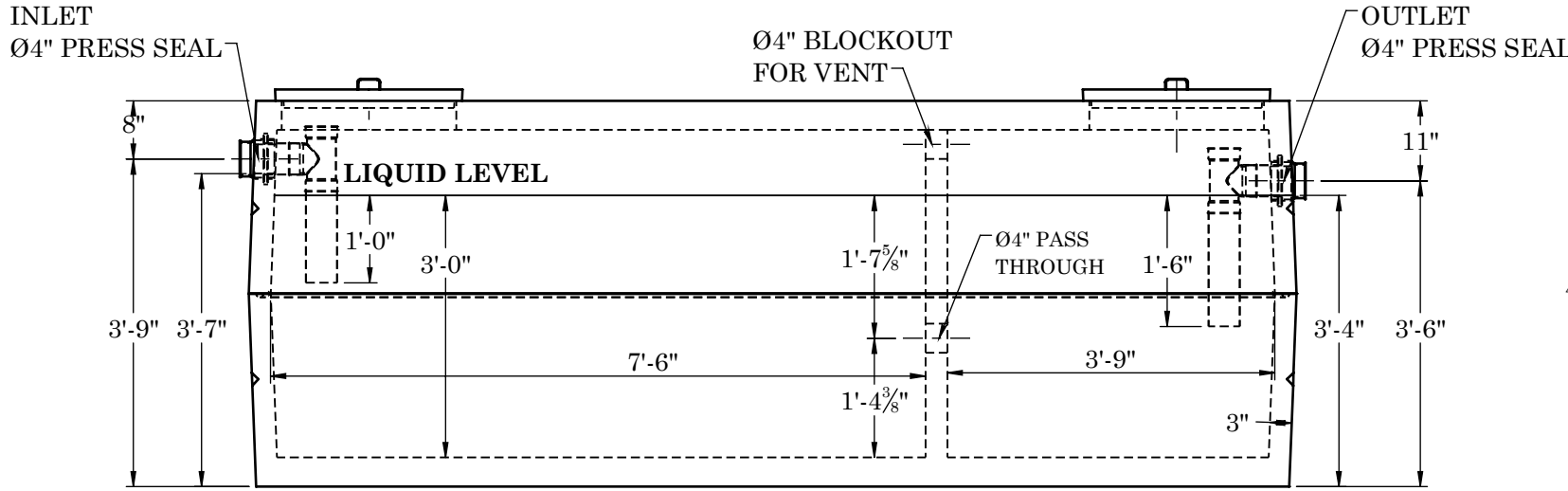
FRONT VIEW
