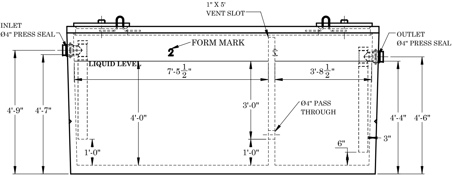
FRONT VIEW
