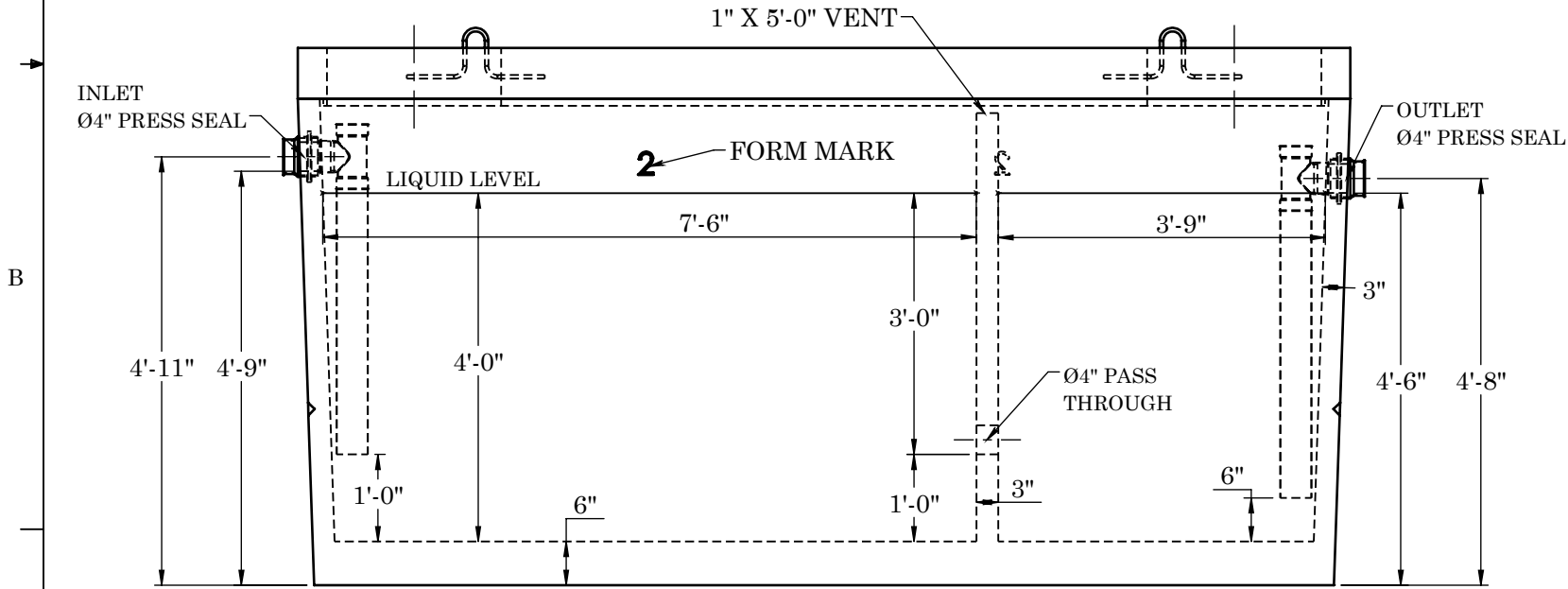
FRONT VIEW
