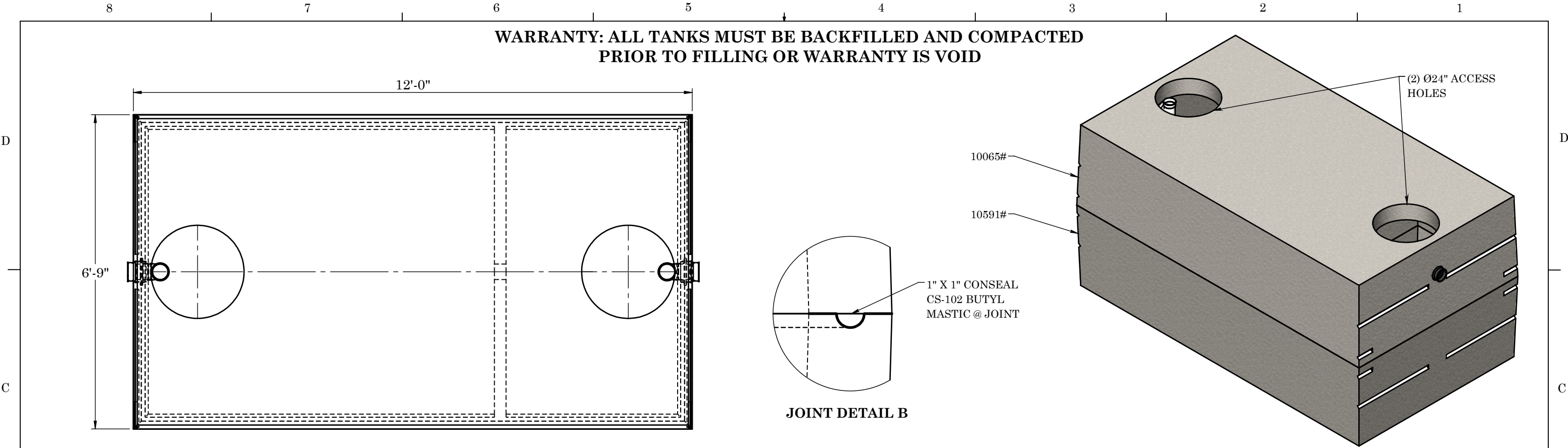
TOP VIEW
