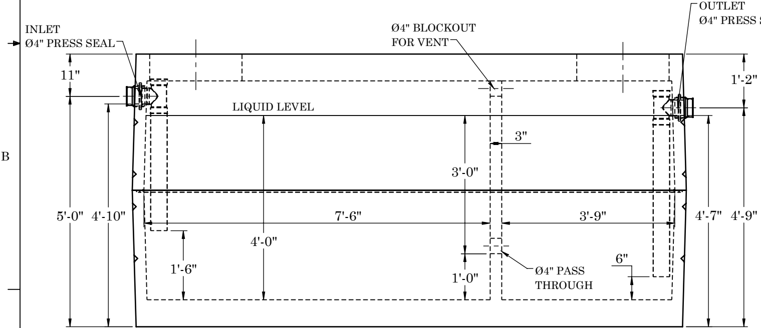
FRONT VIEW
