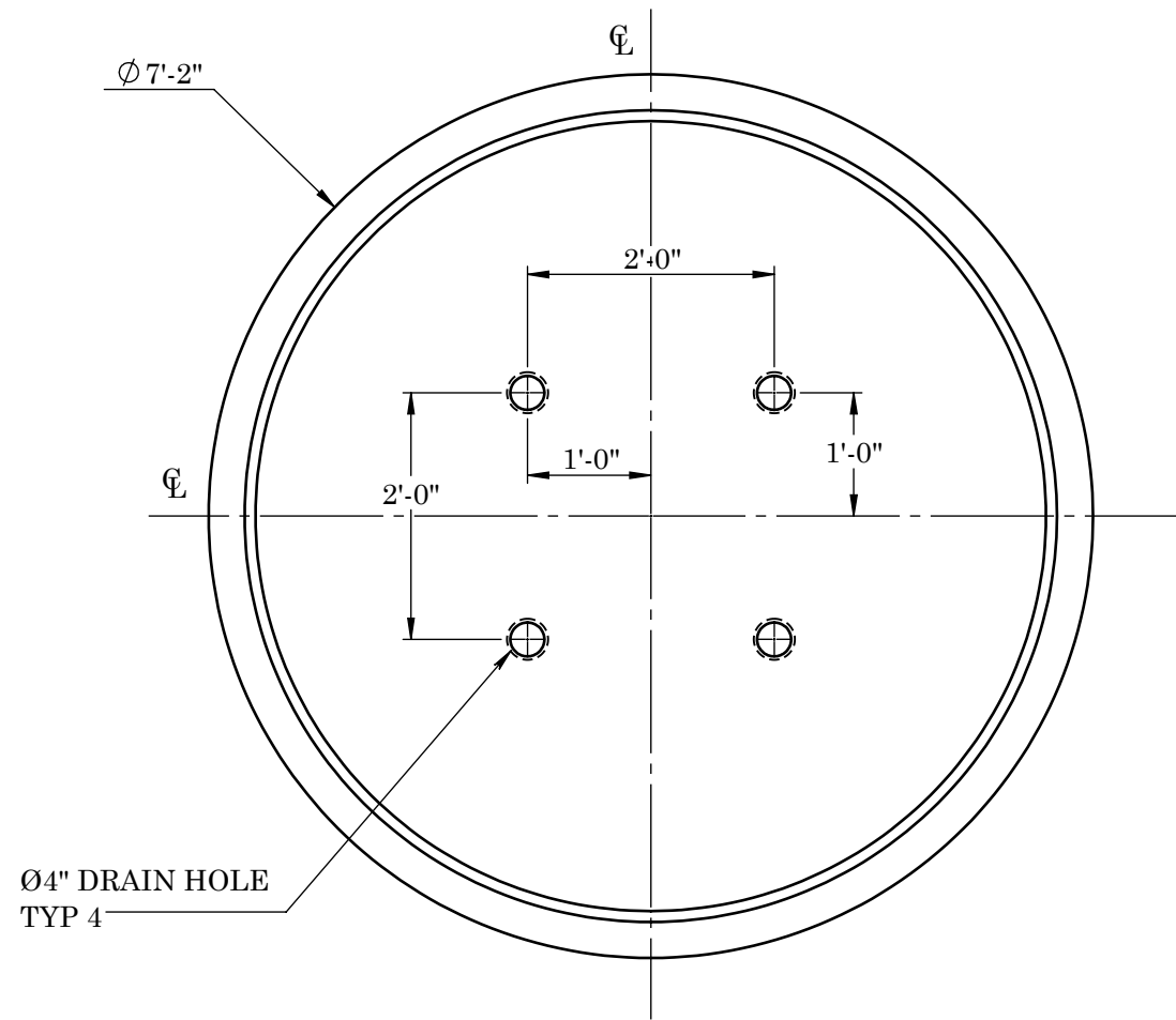
TOP VIEW
