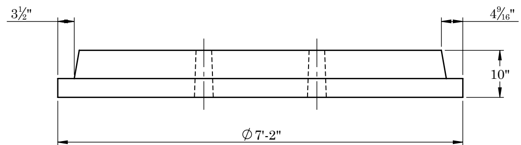
RIGHT VIEW
