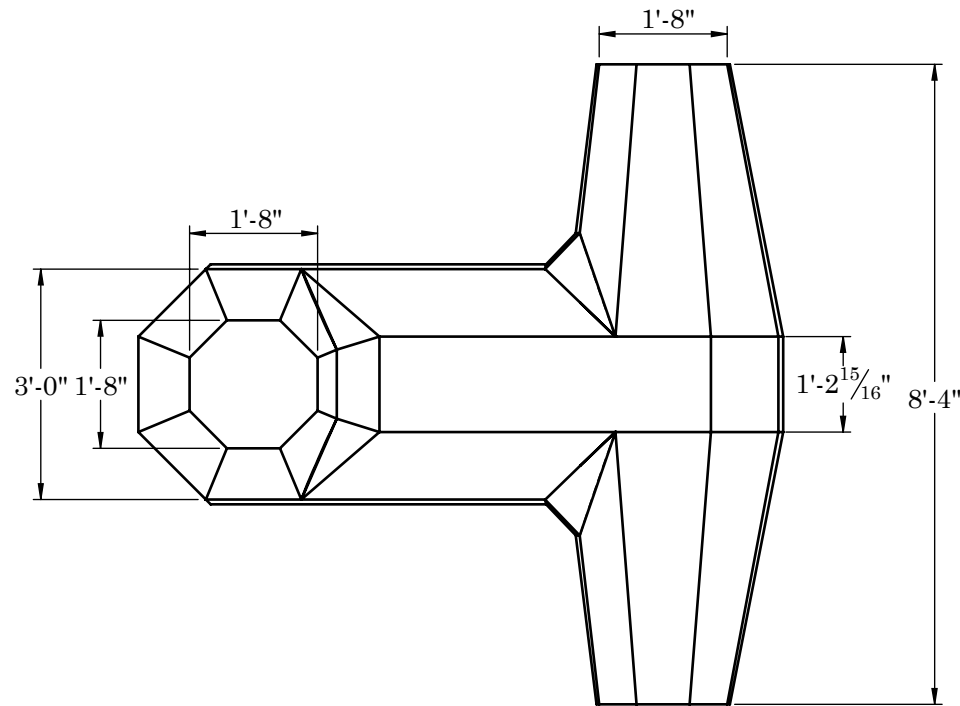
RIGHT VIEW
