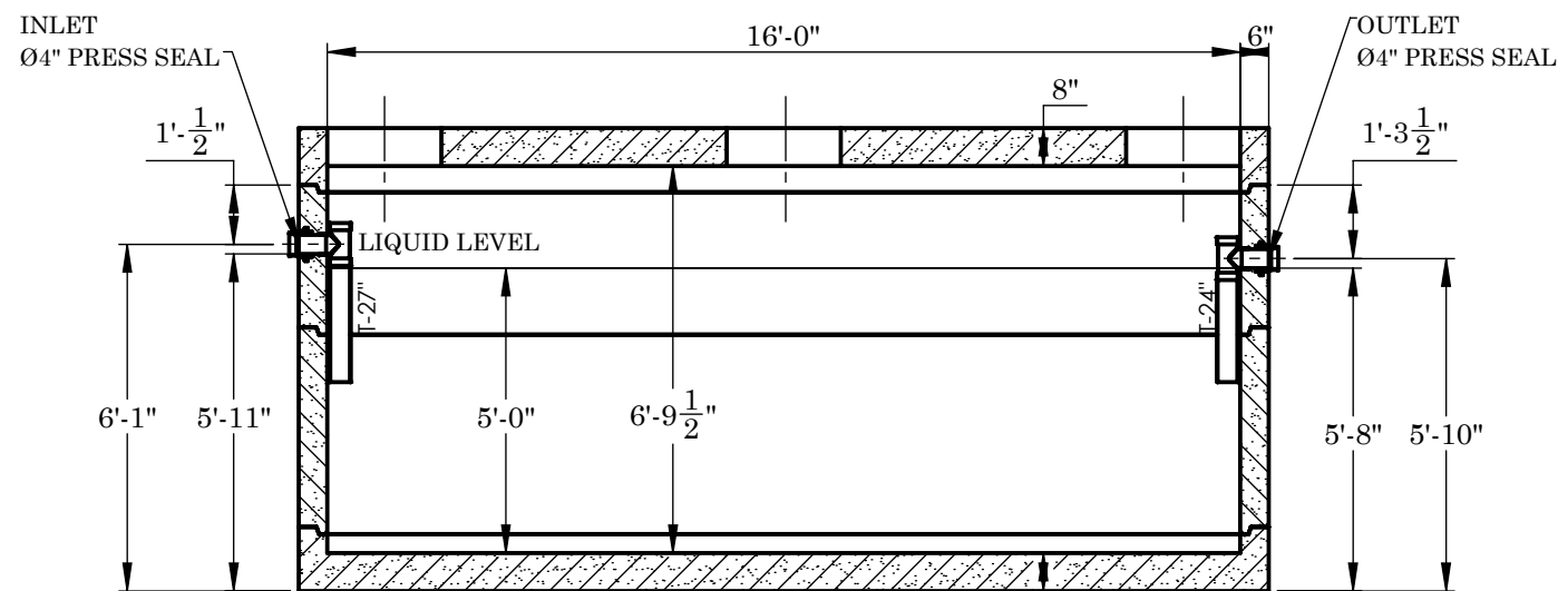
FRONT SECTION VIEW A-A
