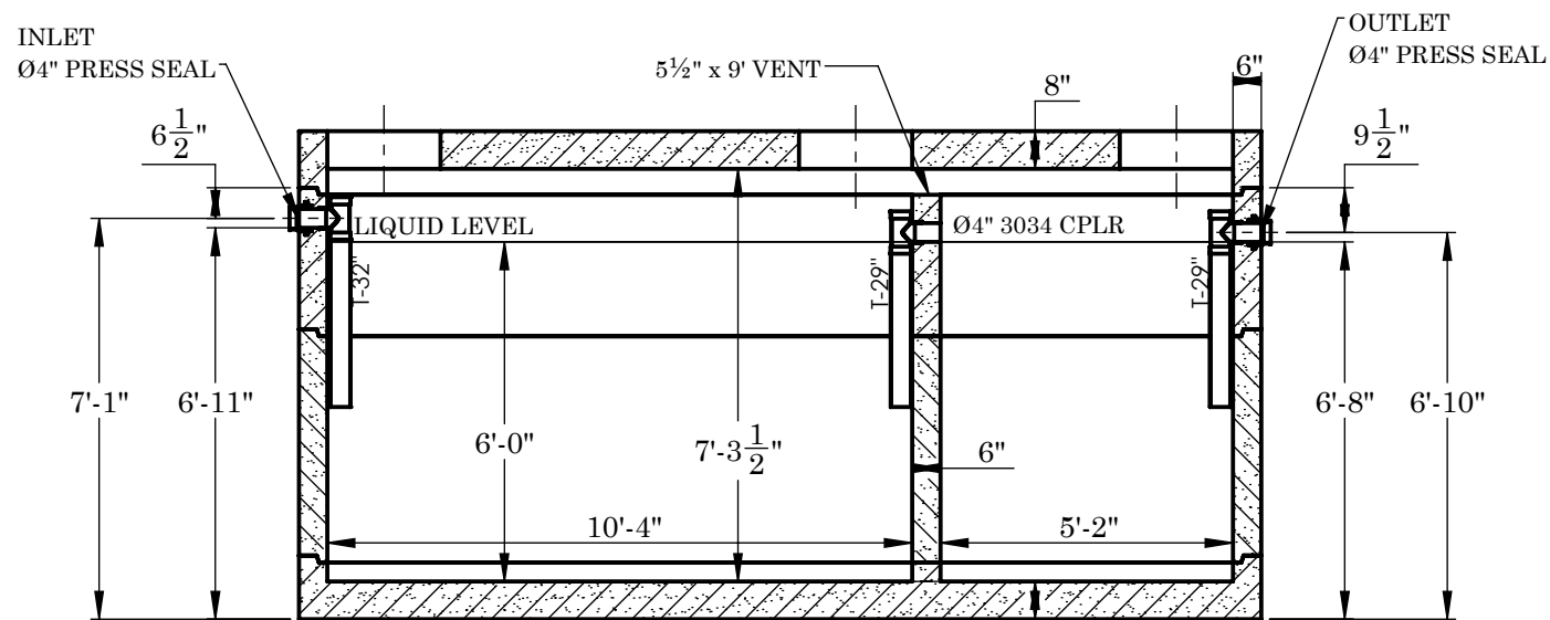
FRONT SECTION VIEW A-A
