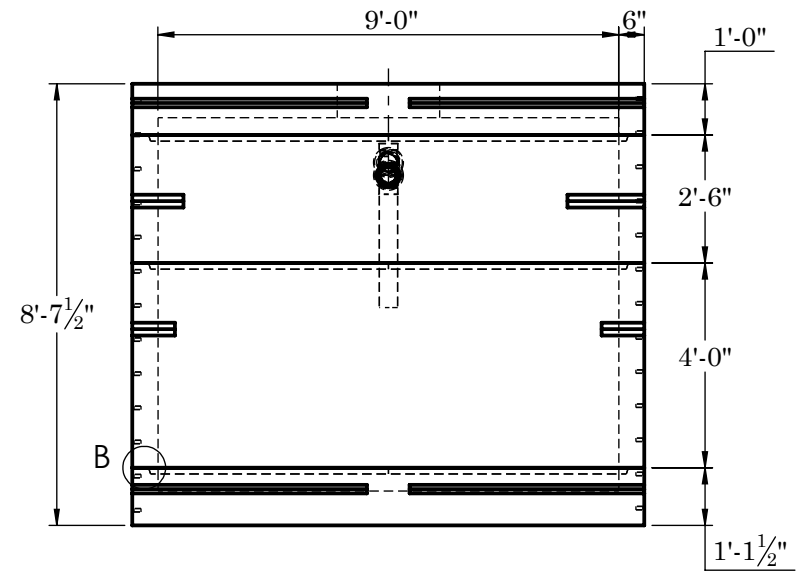
RIGHT VIEW
