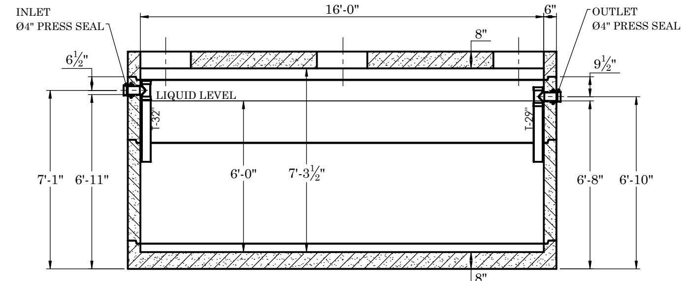
FRONT SECTION VIEW A-A
